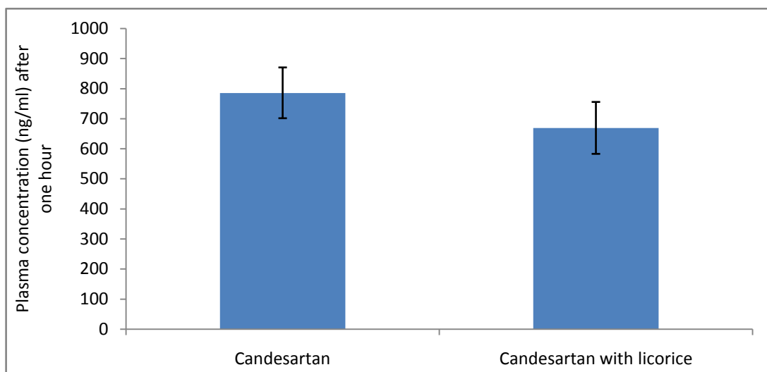
Figure 22: Diagram with error bars comparing the mean (with its 95% confidence interval) serum candesartan drug concentration after one hour of drug administration between single and combined drug use.
